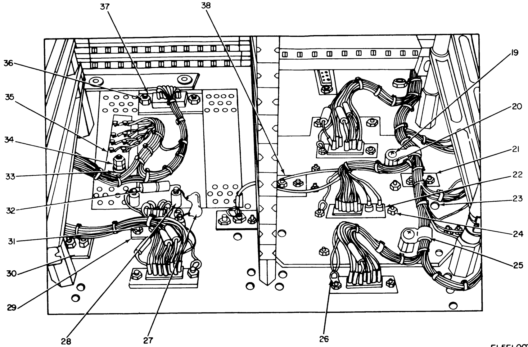
Figure 5. Test Set, Electronic Circuit Plug-In Unit AN/ARM-87, Chassis Assembly, Bottom View (Sheet 2 of 2).
