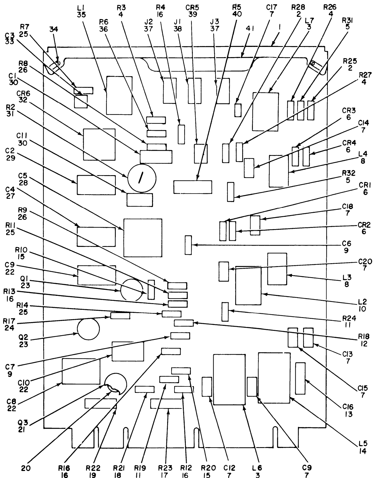
Figure 13. Test Set, Electronic Circuit Plug-In Unit AN/ARM-87, 500-KHz FM Oscillator.
