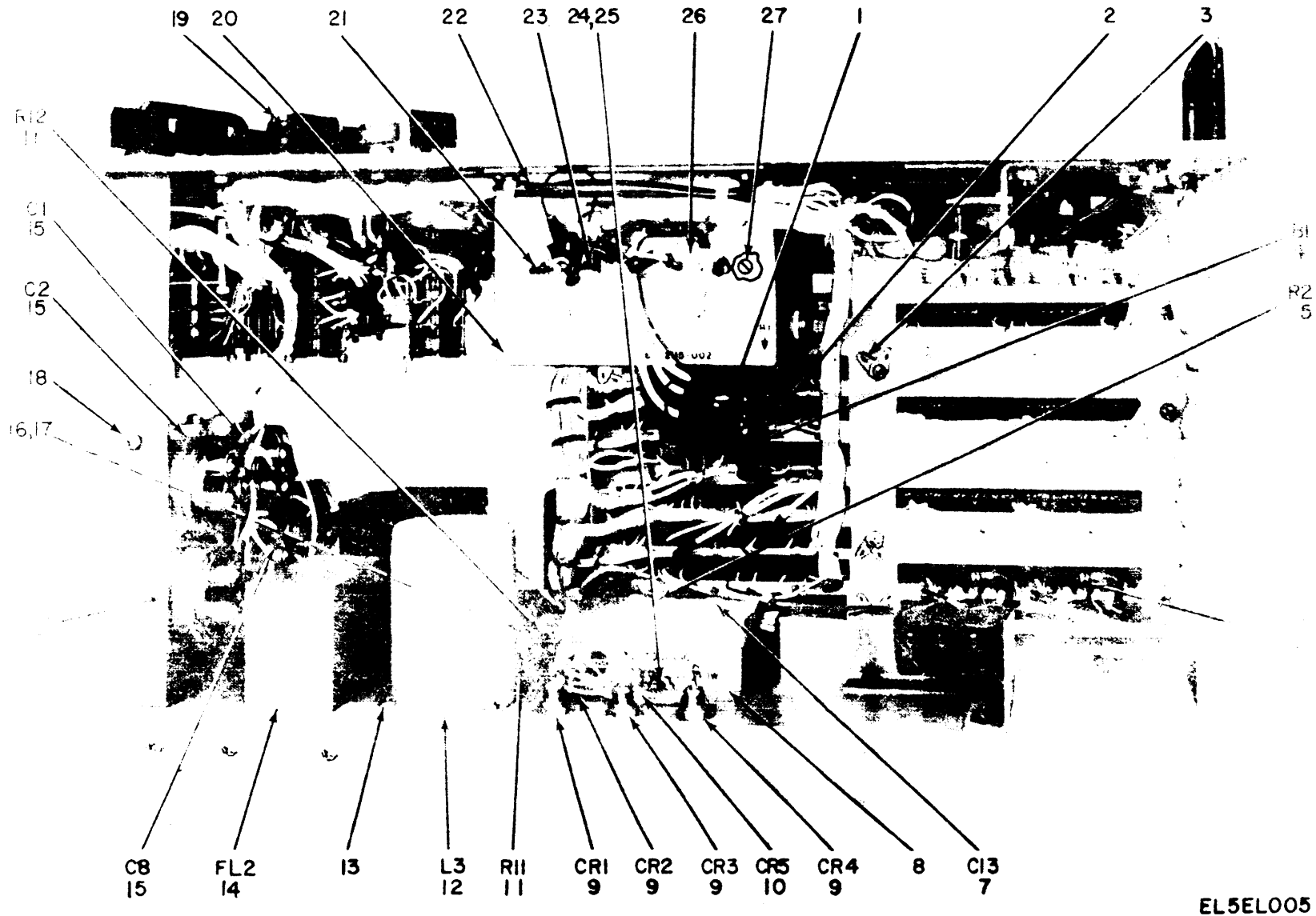
Figure 4. Test Set, Electronic Circuit Plug-In Unit AN/ARM-87, Chassis Assembly, Top View.
