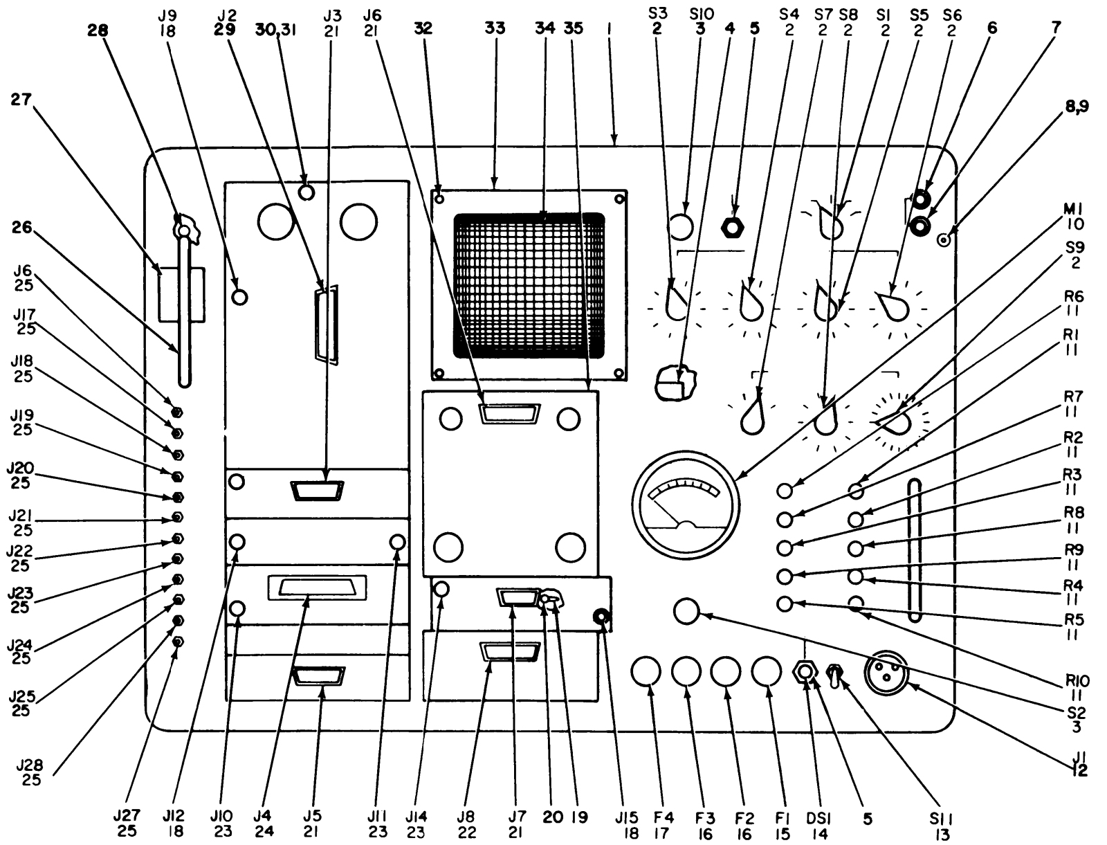
Figure 2. Test Set, Electronic Circuit Plug-In Unit AN/ARM-87, Front Panel.
