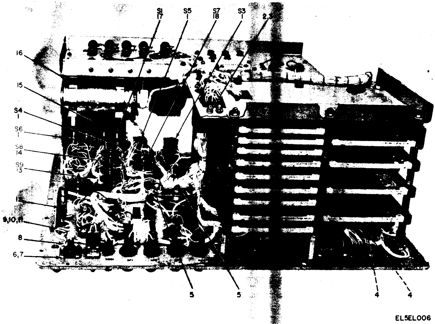
Figure 5. Test Set, Electronic Circuit Plug-In Unit AN/ARM-87, Chassis Assembly, Bottom View (Sheet 1 of 2).
