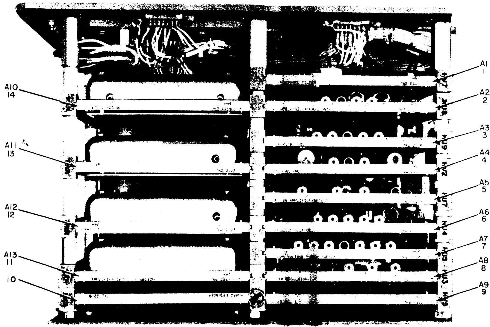
Figure 9. Test Set, Electronic Circuit Plug-In Unit AN/ARM-87, Plug-In Modules.
