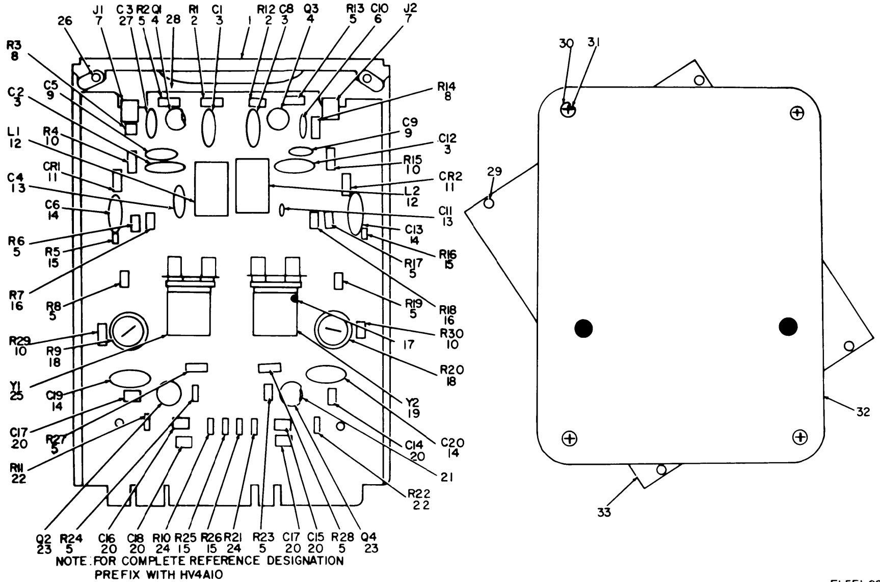
Figure 19. Test Set, Electronic Circuit Plug-In Unit AN/ARM-87, 3.975/5.925-MHz Oscillator.
